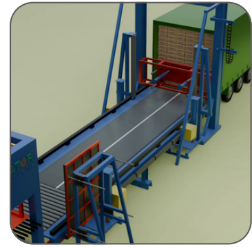
Load Plate
